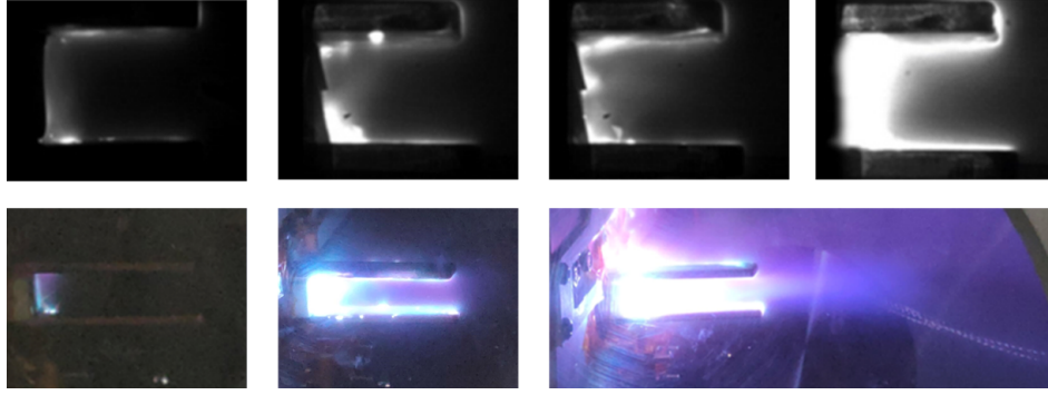
Figure 1: Two different sequences of an APPT discharge sequences. Discharge Channel height 1 cm. The discharge evolves from a plasma seed travelling towards the anode, leading to the ignition of the main channel. Canting 9 of the plasma sheet and some hot spots 10 on the electrodes are also visible. Plasma concentrates towards the electrode edges, agreeing with the deposition patterns on the electrodes reported in the literature. 11
