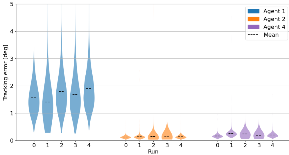
Figure 5: Violin plot of DRL agent mean tracking error during last 50 s of episode in 1000 testing episodes of tracking SQUAD trajectories.
