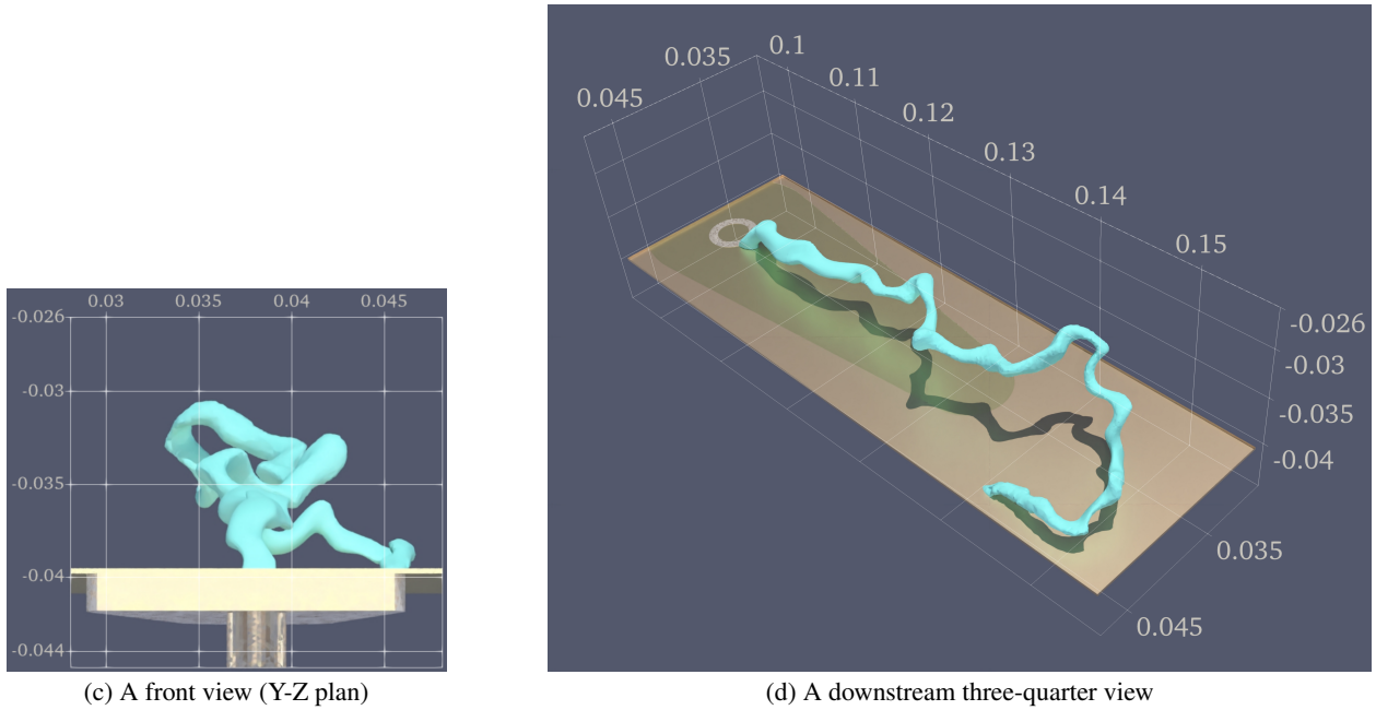
Figure 6: Structure of the arc visualized with contour plot for T = 8\,000\text{ K} and 68\text{ }\mu\text{s} after plasma ignition. All quantities are meters
