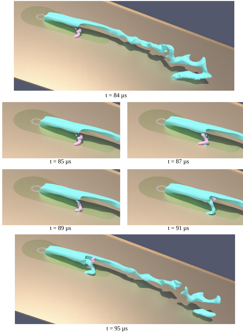
Figure 13: Mechanism of restrike; in blue the current electric arc and in purple the streamer
