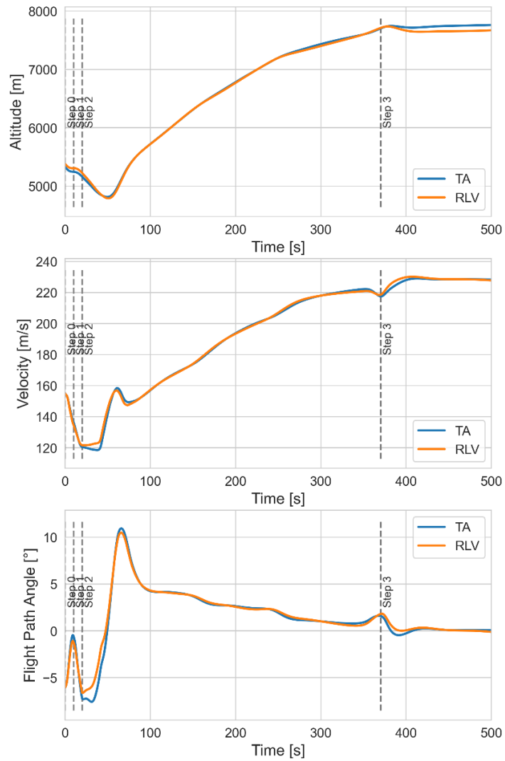
Figure 12: Pull-Up Manoeuvre Trajectory without Wake
