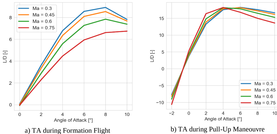
Figure 5: Trimmed Performance Curves for Different TA Configurations in IAC
