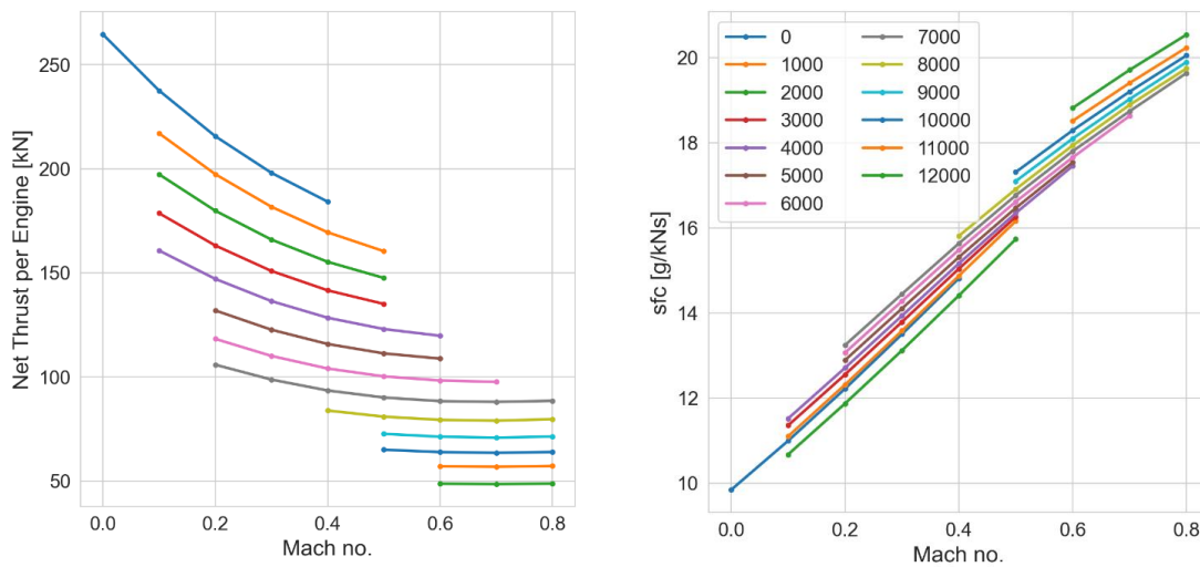
Figure 6: Calculated Performance Maps at Different Altitudes [m] for Rolls Royce Trent-500 at Full Throttle
