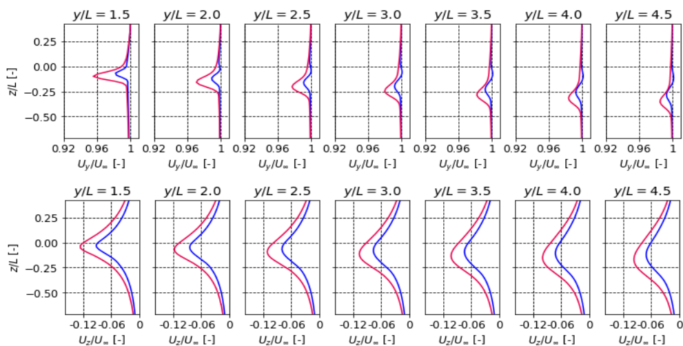
Figure 9: Wake Velocity Components in Fuselage Plane for Aircraft Angle of Attack of 8^\circ (blue) and 12^\circ (red)
