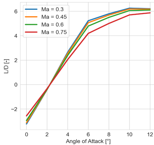
Figure 4: Trimmed Performance Curves of RLV during Pull-Up Manoeuvre
