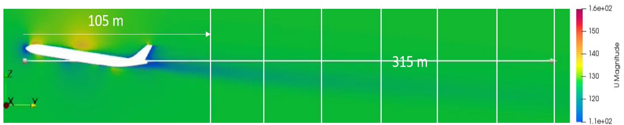
Figure 8: Wake Velocity Magnitude Contours for Angle of Attack of 8^\circ
