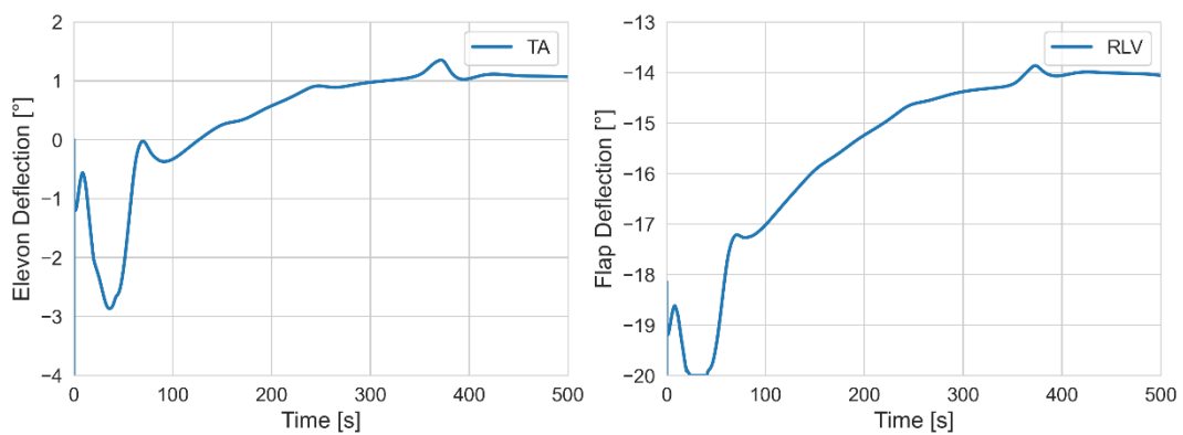
Figure 13: Control Deflection during Pull-Up Manoeuvre: TA (Left) and RLV (Right)
