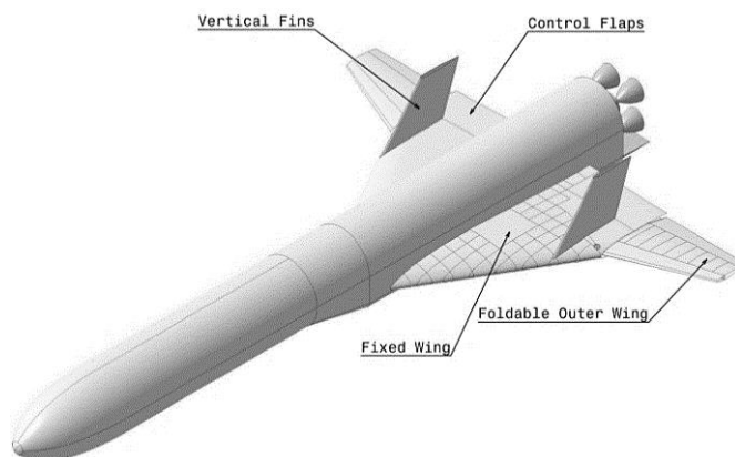
Figure 2: Subsonic Configuration of RLVC4-IIIB [8]
