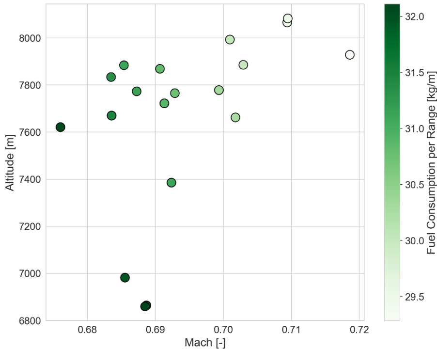
Figure 10: Optimal Cruise Velocity and Altitude based on Fuel Consumption per Range
