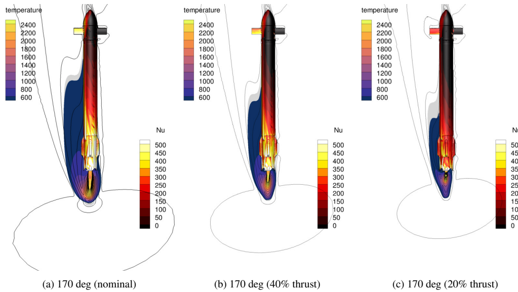
Figure 23: Heat flux on UFO configuration for varying thrust level ( T_w = 300 K, M = 0.8 , \rho = 0.72065 \text{ kg/m}^3 ).
