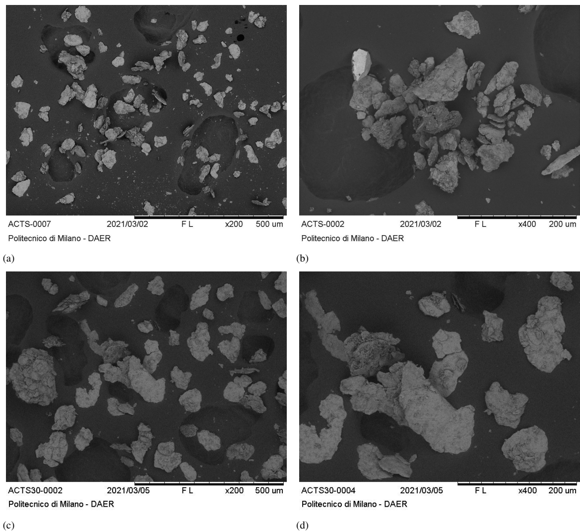
Figure 6: SEM images of (a,b) Act – AlMg – 50, (c,d) Act – AlMg – 70.
