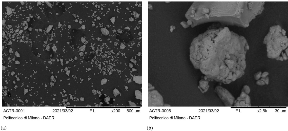
Figure 5: SEM images of the AlMg – 50.
