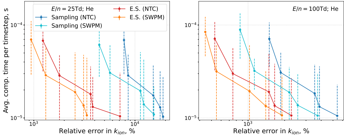
Figure 6: Average computational time per timestep plotted against the relative error in ionization rate coefficient in helium for a reduced field of 25 Td (left) and 100 Td (right). Vertical bars denote a range of \pm 1 standard deviation in the average computational time per timestep.
