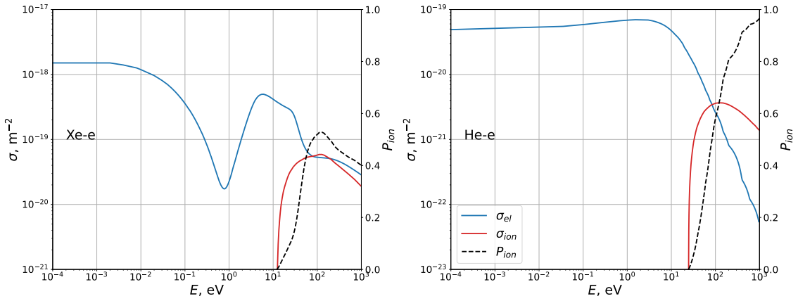
Figure 1: Electron-neutral elastic scattering and ionization cross-sections as a function of the relative translational energy for xenon (left) and helium (right). The dashed line shows the ionization probability as a function of the relative translational energy.
