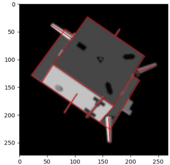
(b) Example of in-view wireframe reprojection in a cropped image of the dataset.
