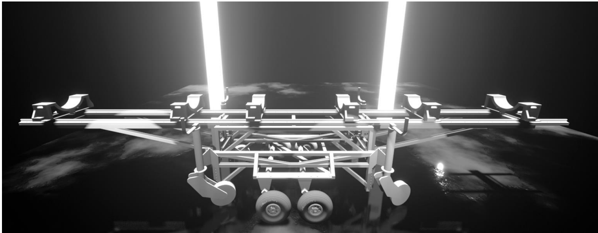
Figure 5: View of kart system for ASTREOS: 6 supports cradles (2 by launcher stage), 4 jockey wheels and 2 car axes
