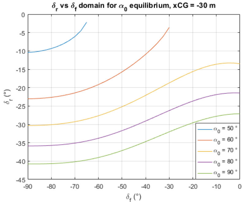
Figure 8 : Front and rear fins angles domain for several equilibrium AoAs
