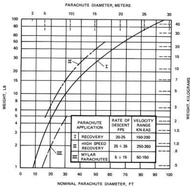
Figure 8: Mass of a nylon main descent parachute 12
