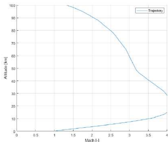
Figure 3: Trajectory of the tank
