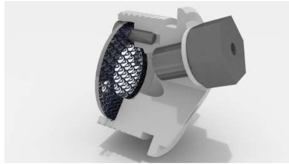
Figure 18: Section view of the Stratos gas generator
