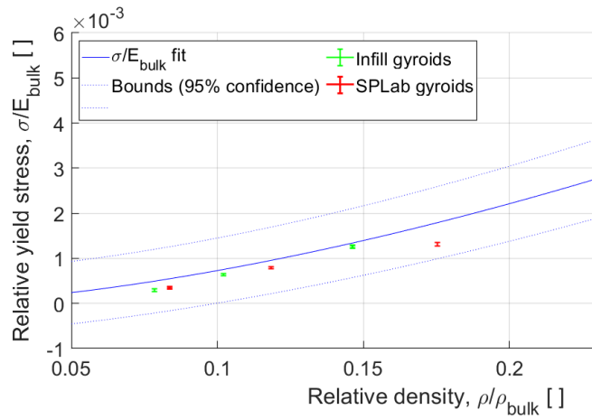
(b) Gyroid relative yield stress vs. relative density
