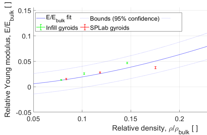
(a) Gyroid relative Young modulus vs. relative density
