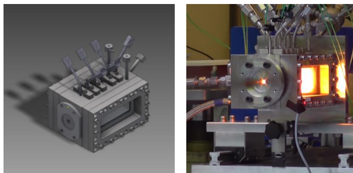
Figure 11: Rectangular gel rocket combustion chamber with optical access (left: sketch; right: hot fire test).
