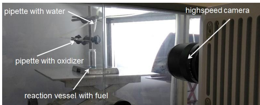
Figure 7: Test setup for drop tests.
