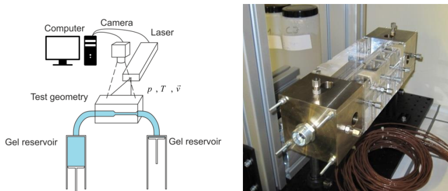
Figure 14: Sketch of test setup for investigation of pressure loss and flow behaviour (left). Measurement section made of acrylic glass (right).
