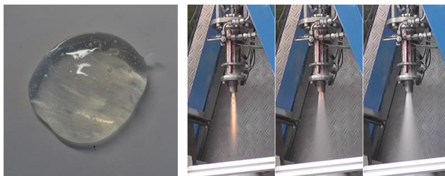
Figure 5: Test sample of a particle free gelled monopropellant (left) and sequence from an ignition test (right)
