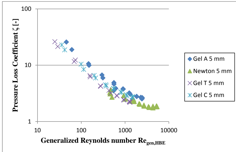
Figure 15: Pressure loss coefficient \zeta with respect to generalized Reynolds number Re_{gen,HBE} in pipe for target diameter d_2=5 mm.
