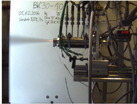
Figure 9: Hot fire test using combustion chamber BK30.
