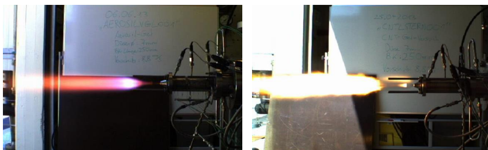
Figure 4: Hot fire test with Aerosil-based gel (left) and a Carbon-based gel (right)
