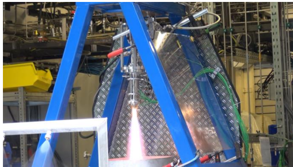
Figure 10: Combustion chamber BK40 is fired at vertical test stand.
