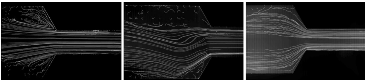
Figure 2: Flow regimes: Gel flow with recirculation areas (left), oscillating flow (middle), gel flow without recirculation areas but high speed near the wall (right)
