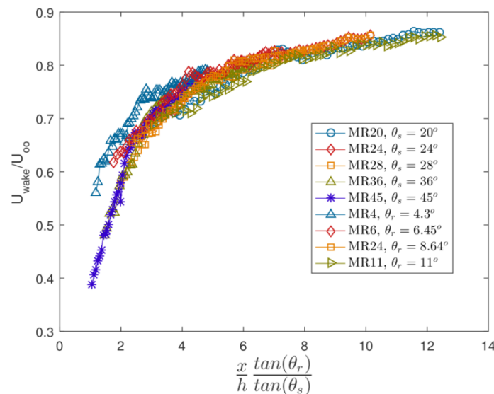
Figure 16: Streamwise evolution of wake velocity with the present scaling.
